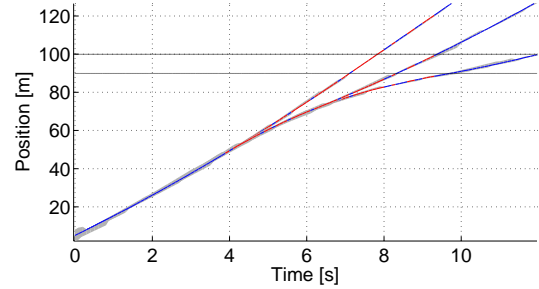
Fig. 2. The real position (union of blue and red) and the position estimate (in grey) of 3 agents over time. Blue lines indicate that the desired inputs are used, red lines that the safe inputs are used.
